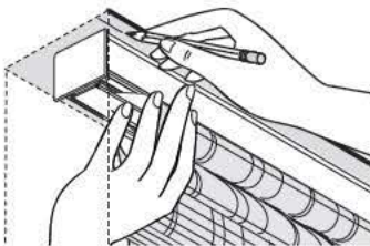
Inside/Ceiling Mount
